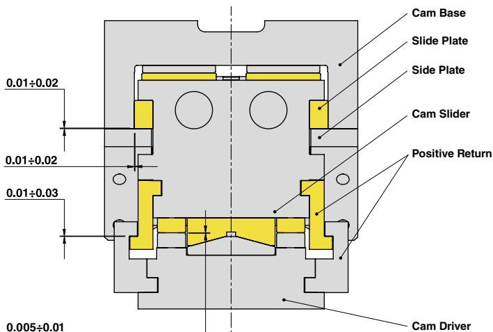
SLIDER STRUCTURE, POSITIVE RETURN STRUCTURE AND CLEARANCES
